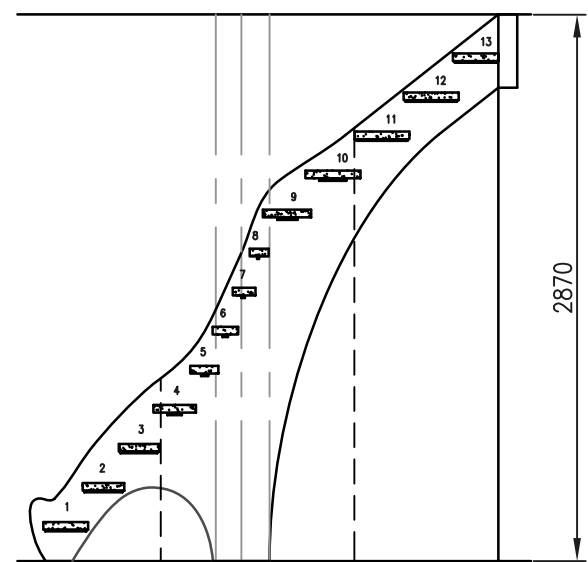
OUTER STRINGER
