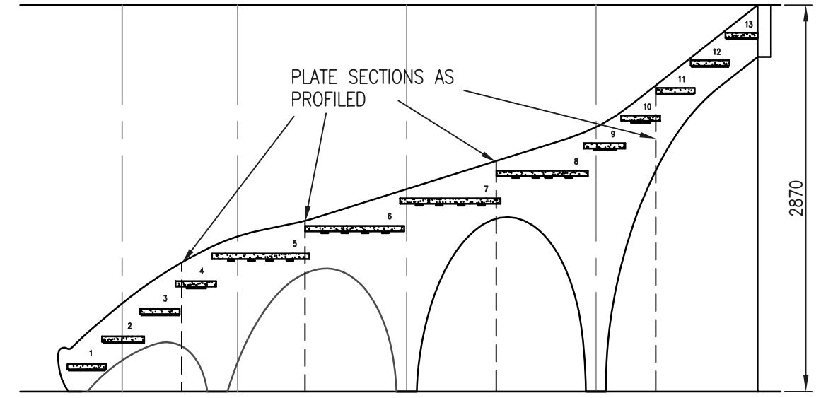
OUTER STRINGER
